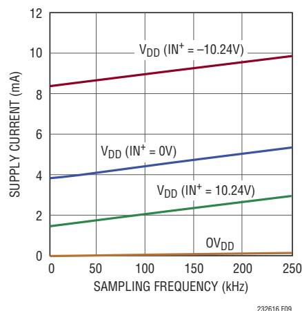
Figure 9. Power Supply Current of the LTC2326-16 Versus Sampling Rate
