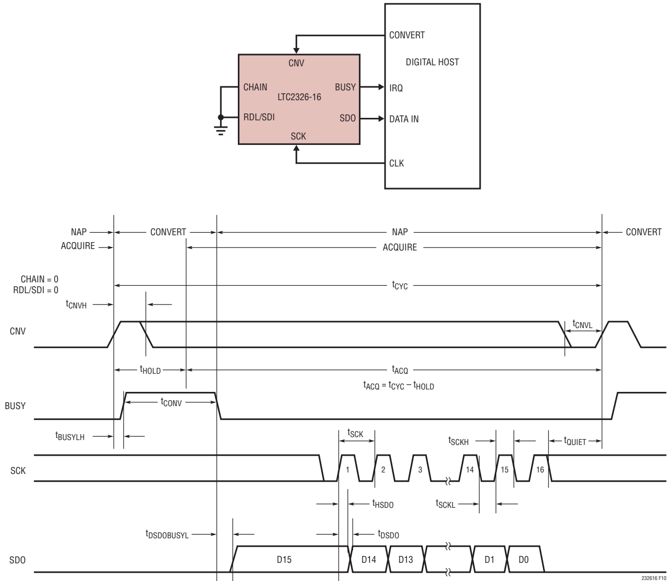
Figure 10. Using a Single LTC2326-16 in Normal Mode
